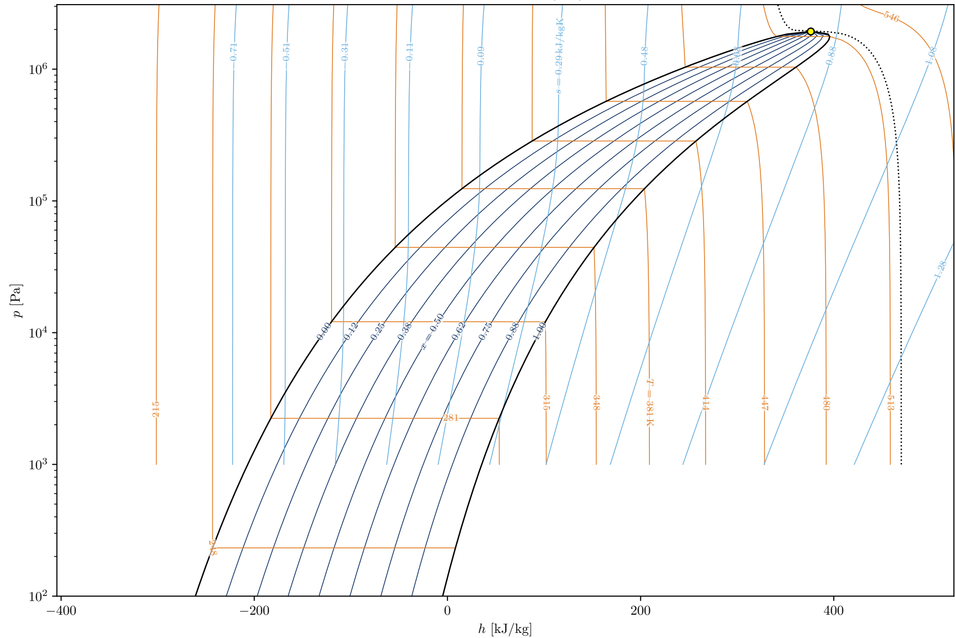
Thermodynamic Diagram (PH) – MM
